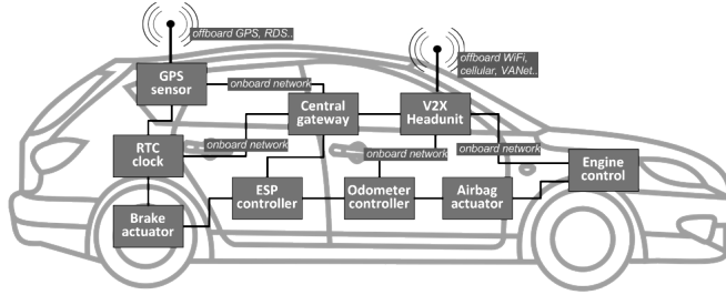
Figure 4: Architecture of connected vehicle [37].
