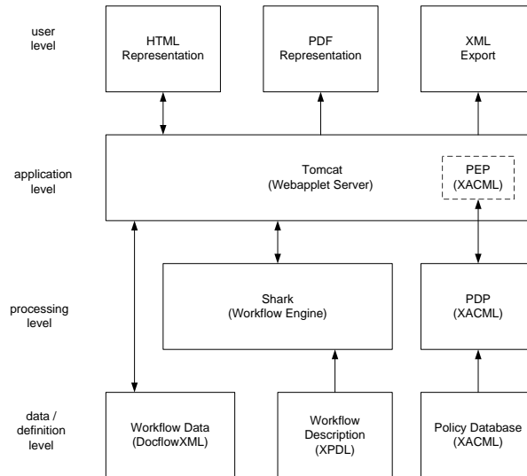
Fig. 3. Framework Overview
