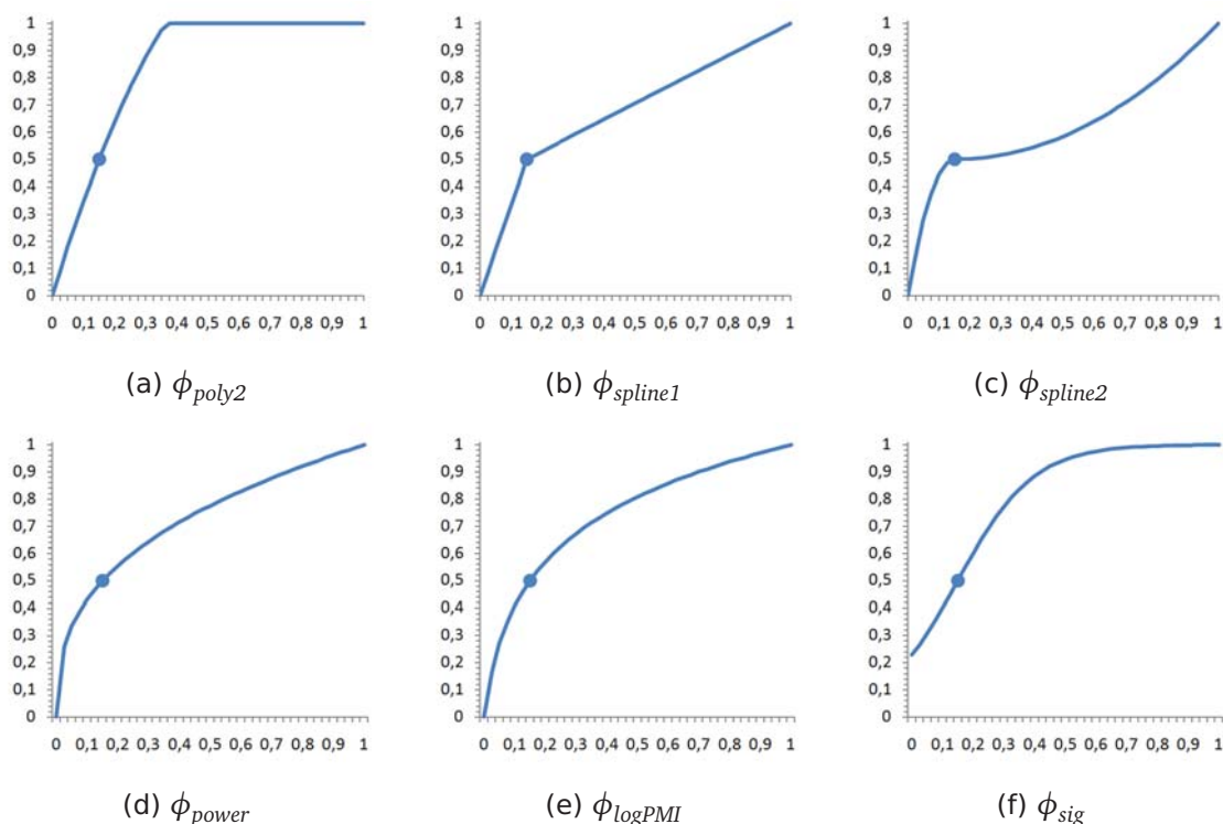
Figure 4.4: Graph of the 6 scaling functions for a threshold \theta of 0.15
