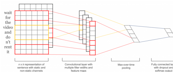
Figure 2: CNN architecture by Kim (2014).
