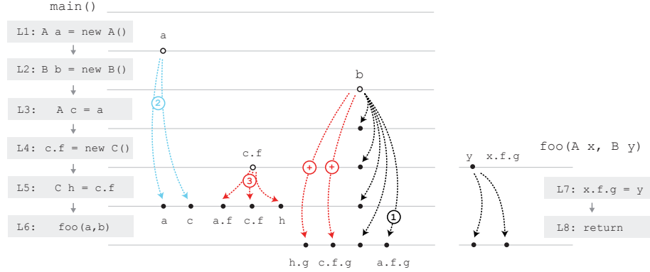
■ Figure 7 Handling aliases on forward return-flow [Return].
