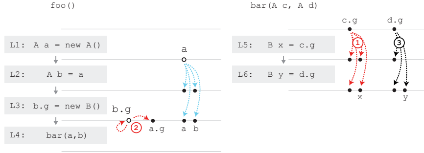
■ Figure 9 Client-Driven Context-Resolution
