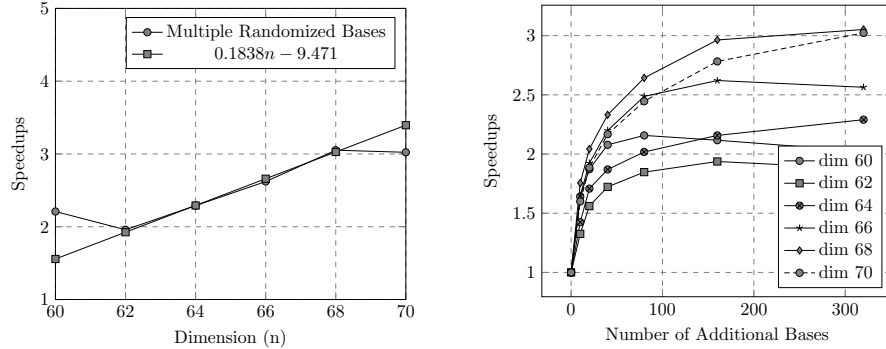
Fig. 6. Speedups with respect to the dimension (left) and the number of additional bases used to seed the list before sieving (right).
