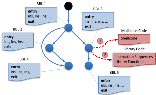
Figure 1: Schematic overview of control-flow attacks
