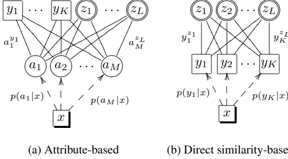
Figure 2. Two models for zero-shot object classification. See Section 3 for discussions.
